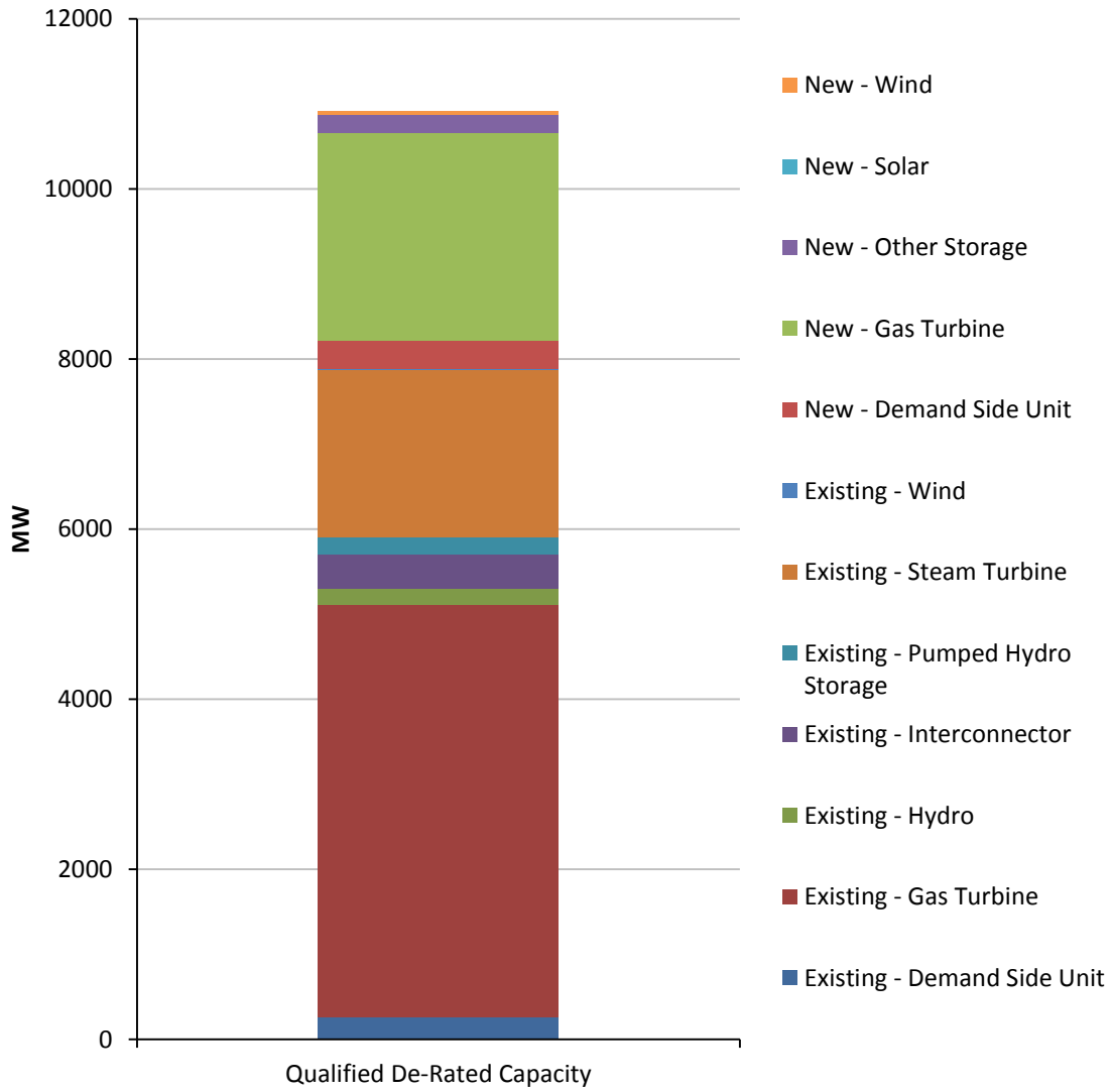
Figure 1 - New and Existing Qualified Capacity by Technology Class
