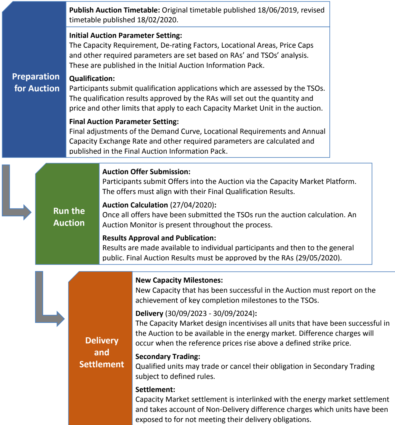
Figure 1: Simplified overview of some of the key processes of the Capacity Market. Some dates relevant to this 2023/2024 T-4 Capacity Auction are also provided.
