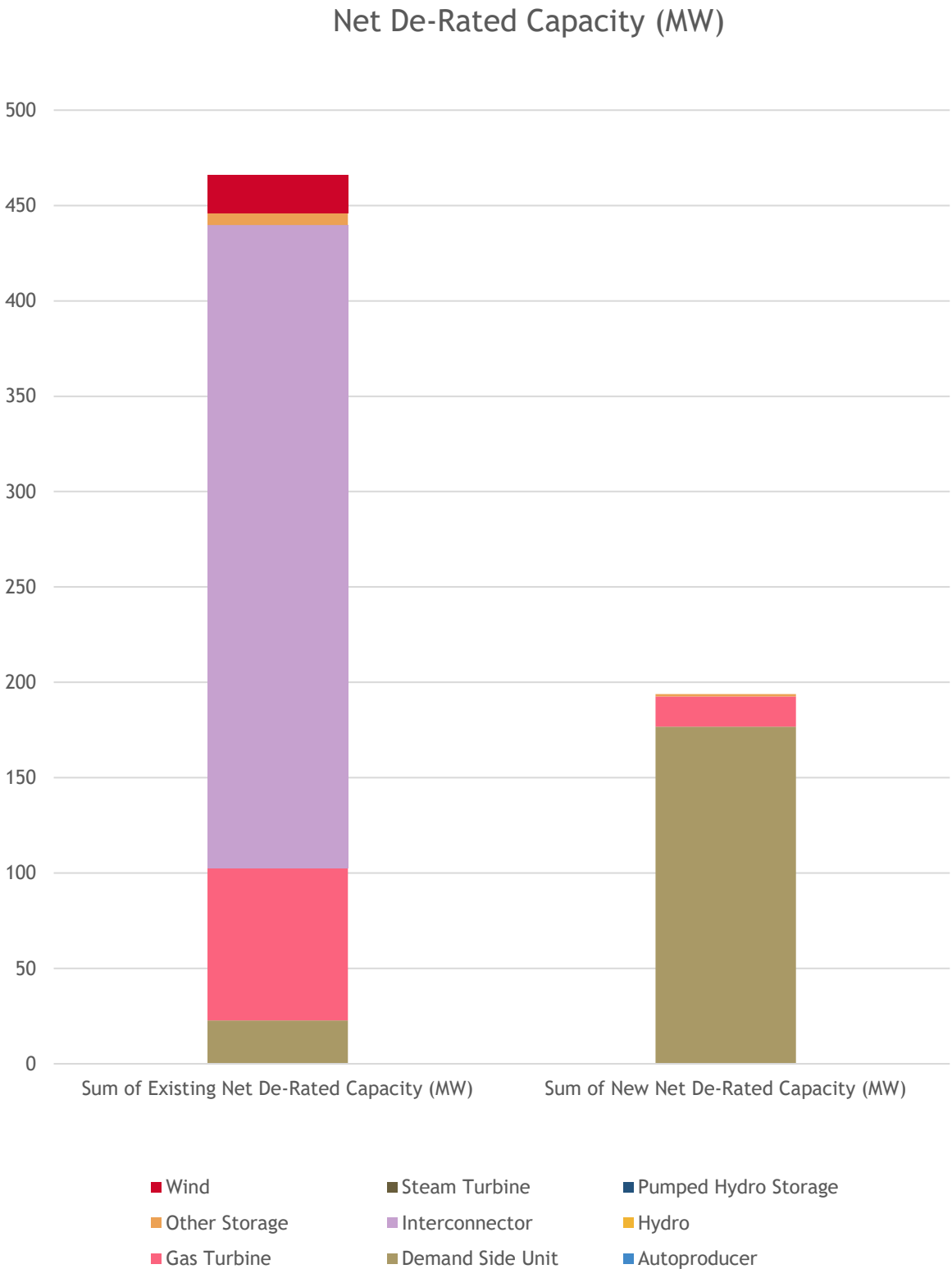
Figure 1 shows the New and Existing Qualified Net De-Rated Capacity by Unit Type/Technology Class for the 2025/2026 T-1 Capacity Auction.
